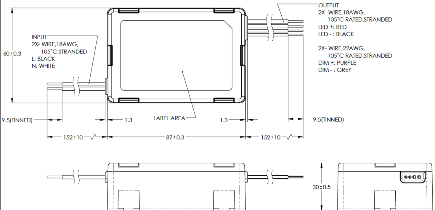
All dimensions are in mm
